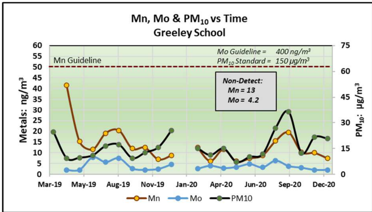
Figure 4: Greeley School – Mn, Mo & PM 10
