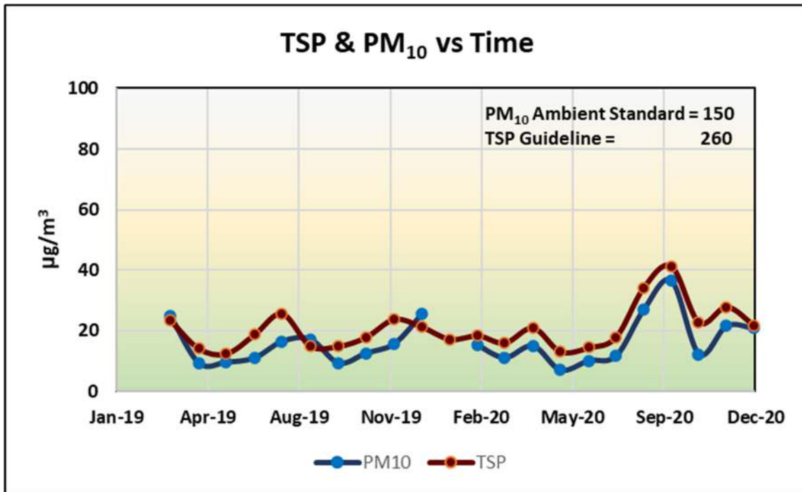
Figure 2: Greeley School – TSP & PM 10
