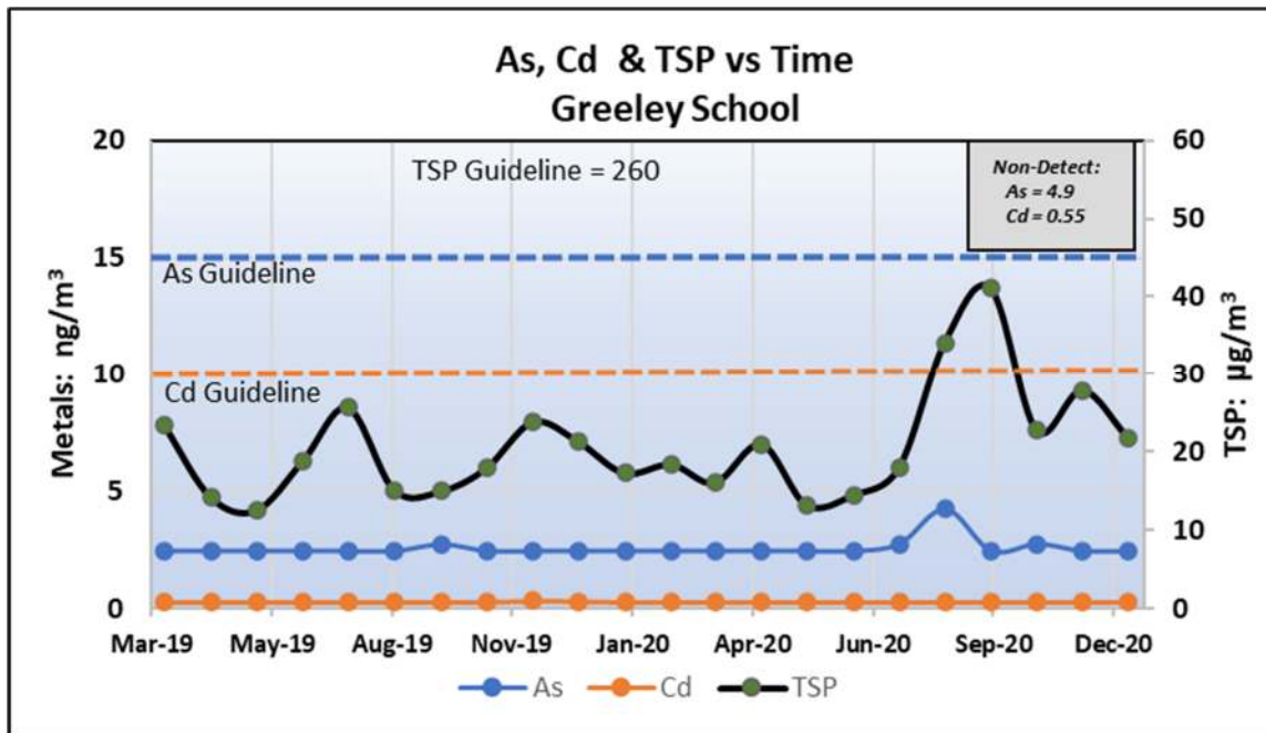
Figure 6: Greeley School – As, Cd & TSP
