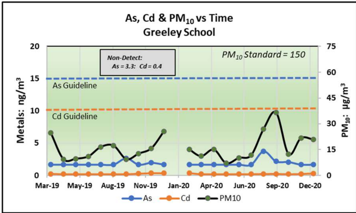
Figure 3: Greeley School – As, Cd & PM 10
