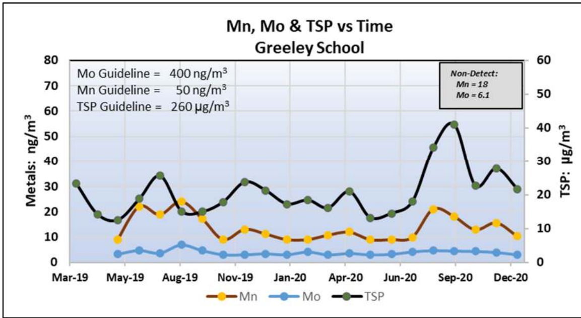
Figure 7: Greeley School – Mn, Mo & TSP
