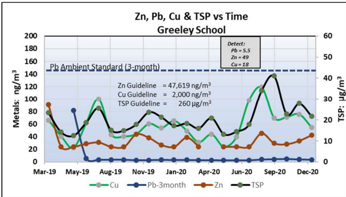
Figure 8: Greeley School – Zn, Pb, Cu & TSP
