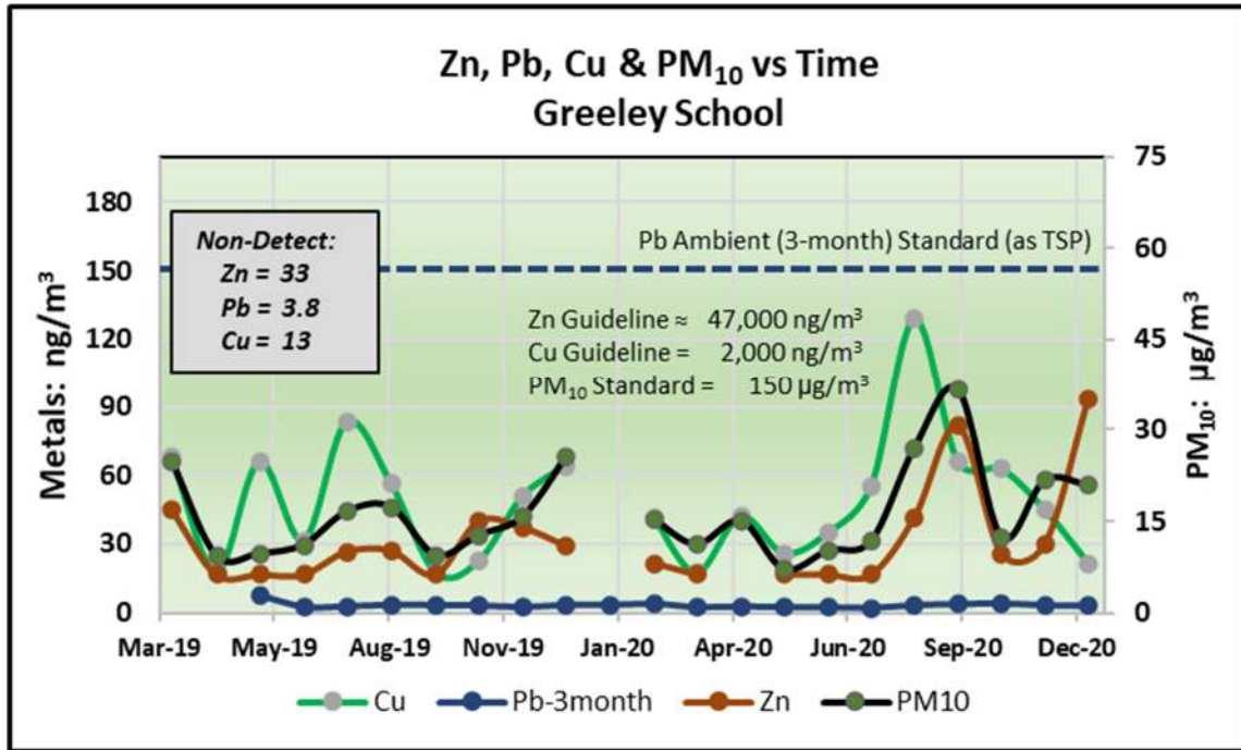
Figure 5: Greeley School – Zn, Pb, Cu & PM 10
